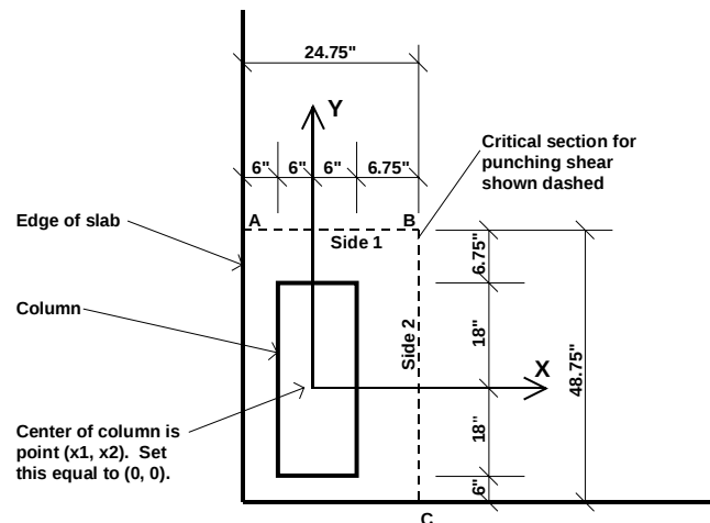
Figure 8: Corner Column, Point 5 in SAFE Model
