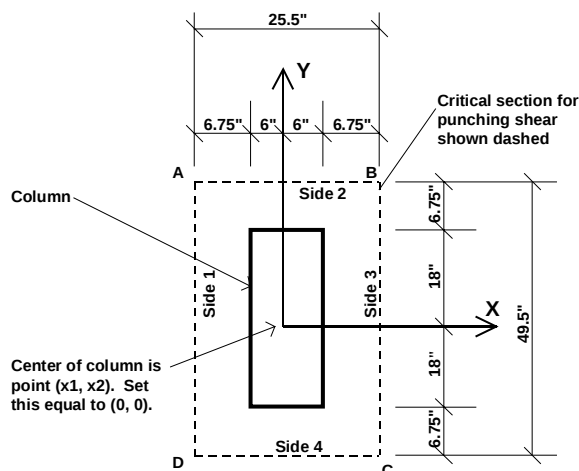
Figure 5: Interior Column, Point 10 in SAFE Model
