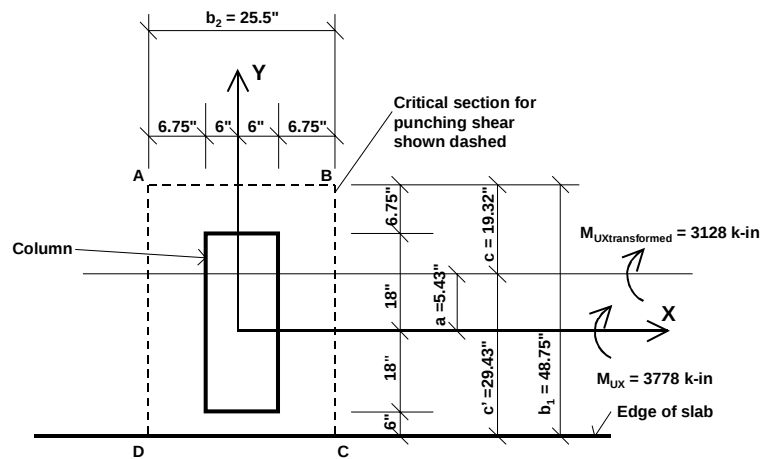
Figure 11: Edge Column With Edge Parallel To X-Axis Point 6 in SAFE Model, Bending About X-Axis
