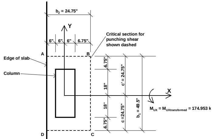
Figure 13: Edge Column With Edge Parallel To Y-Axis Point 9 in SAFE Model, Bending About X-Axis
